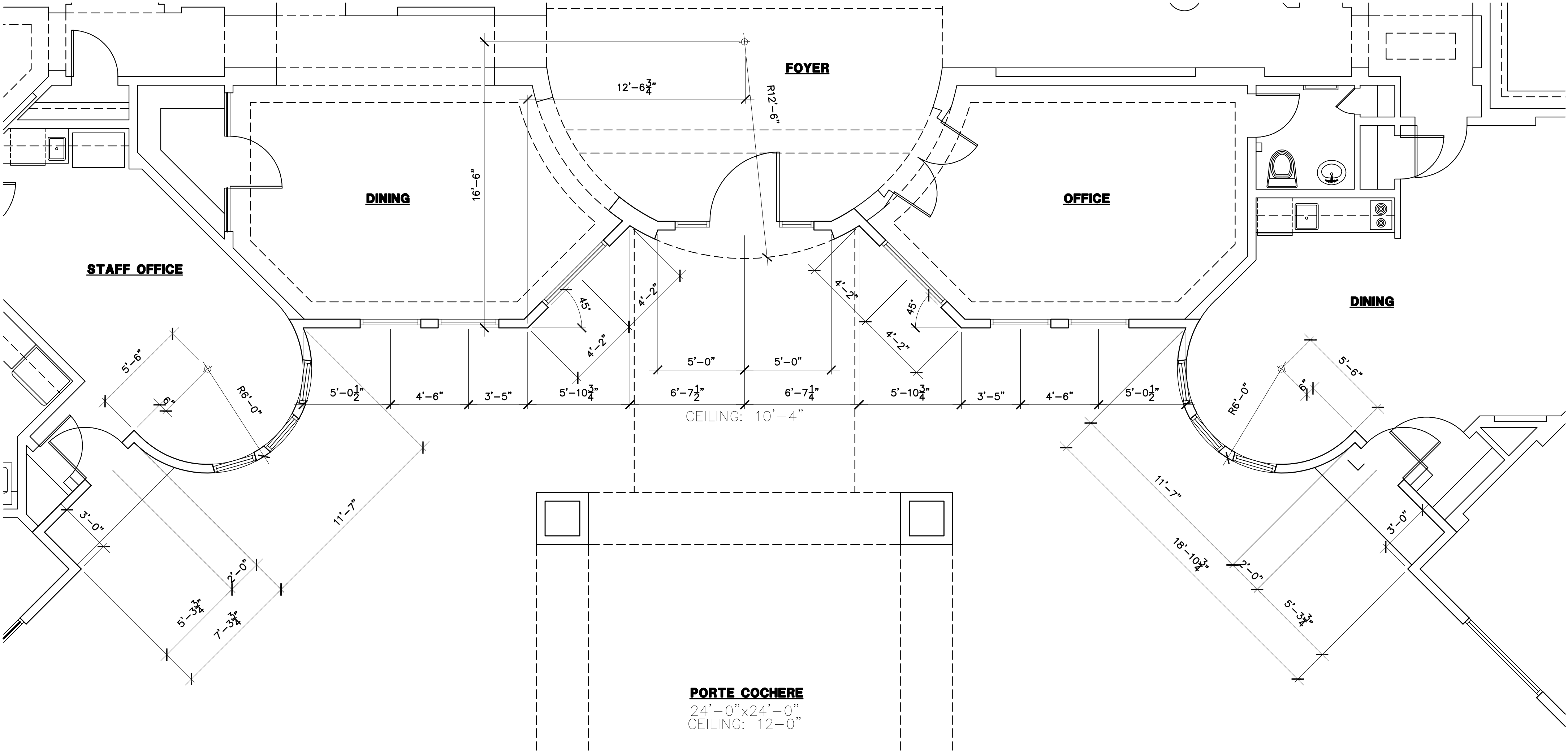
③ ENLARGED DIMENSION PLAN SCALE: 1/4" = 1'-0"
