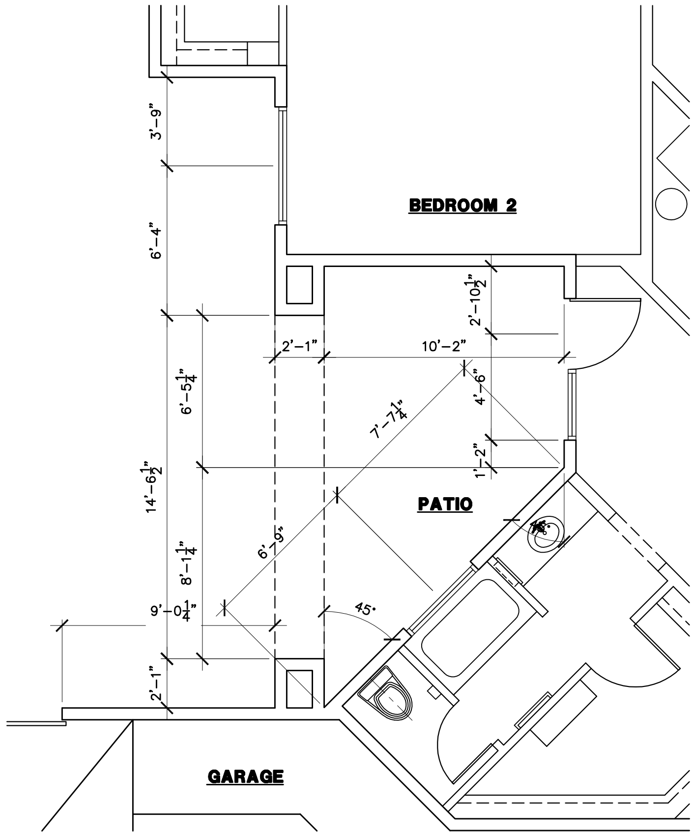
④ ENLARGED DIMENSION PLAN SCALE: 1/4" = 1'-0"
