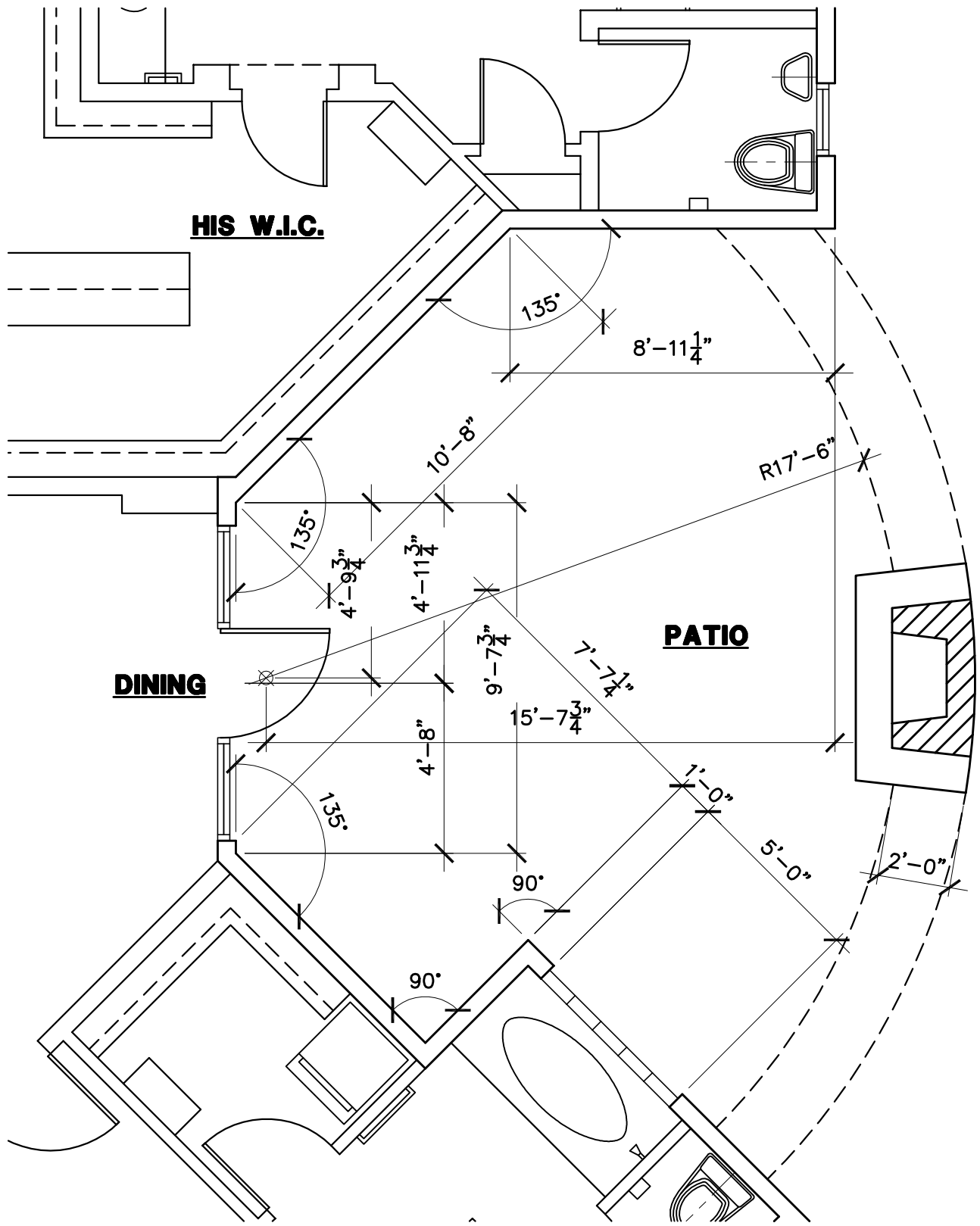
② ENLARGED DIMENSION PLAN SCALE: 1/4" = 1'-0"
