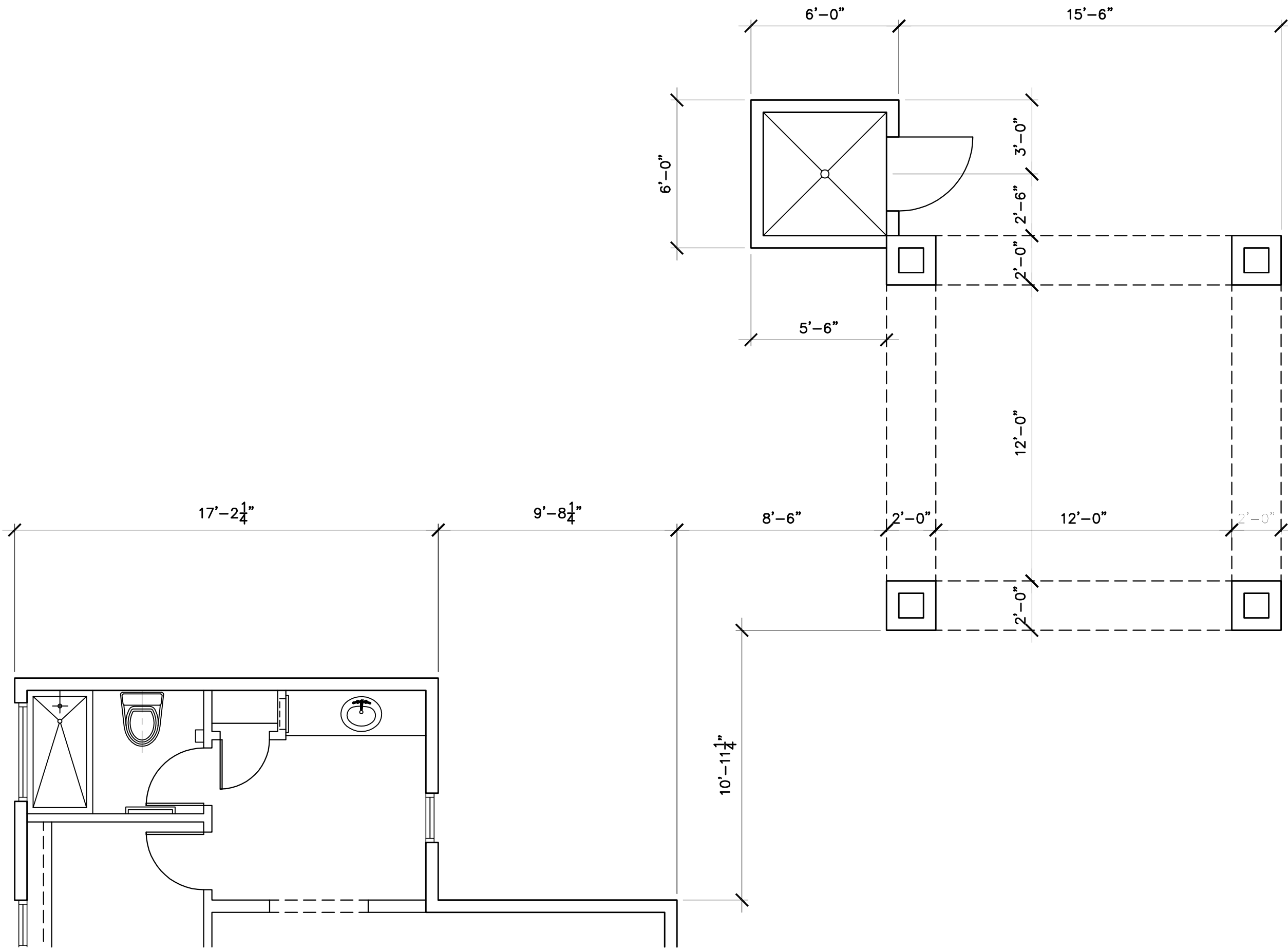
① ENLARGED DIMENSION PLAN SCALE: 1/4" = 1'-0"
